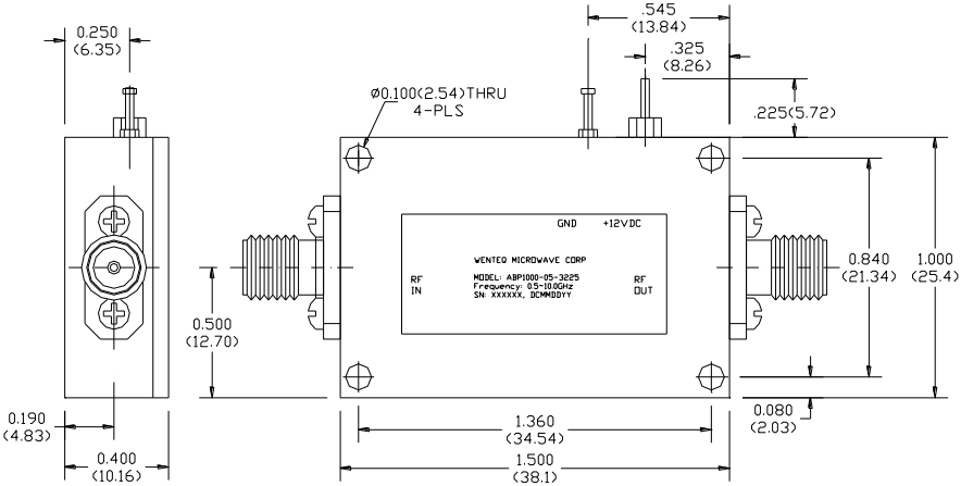
(a) ABP1800-01-3426 amplifier without heatsink
