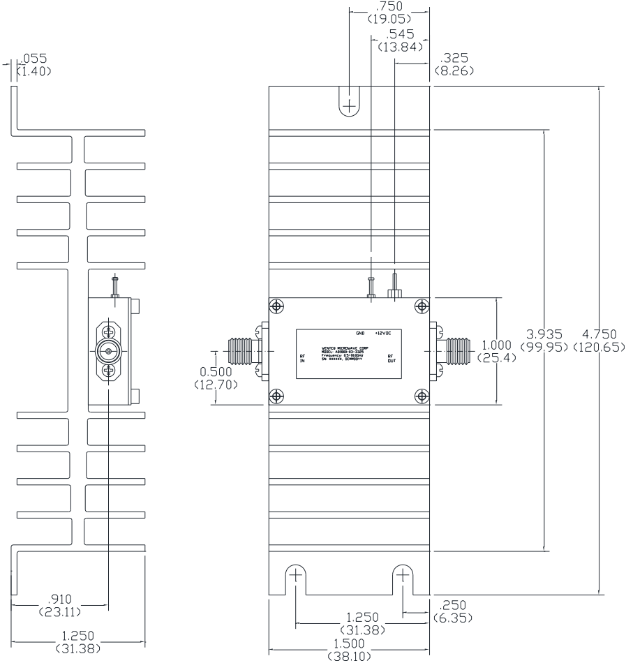
(a) ABP1800-01-3426-X amplifier with heatsink
